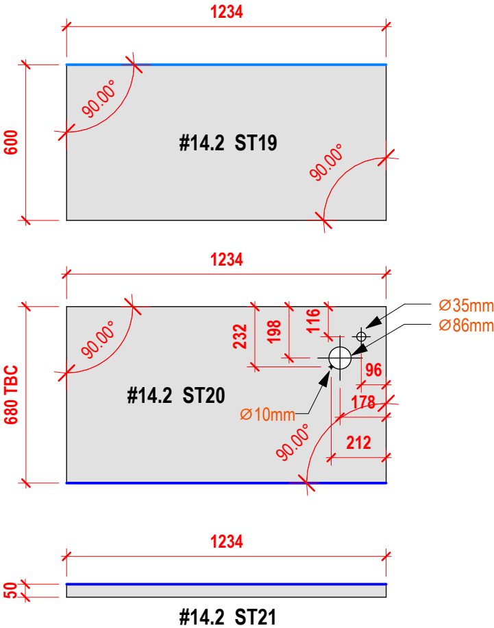
SITTING ROOM - MARBLE BENCHTOP 2 1 : 20
