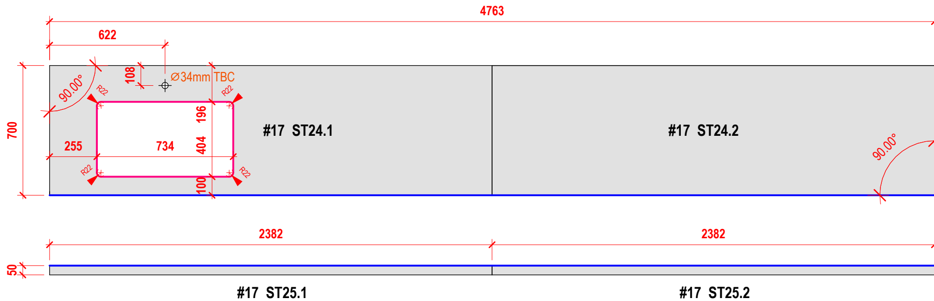
LAUNDRY GF - MARBLE APRON 1 : 20
