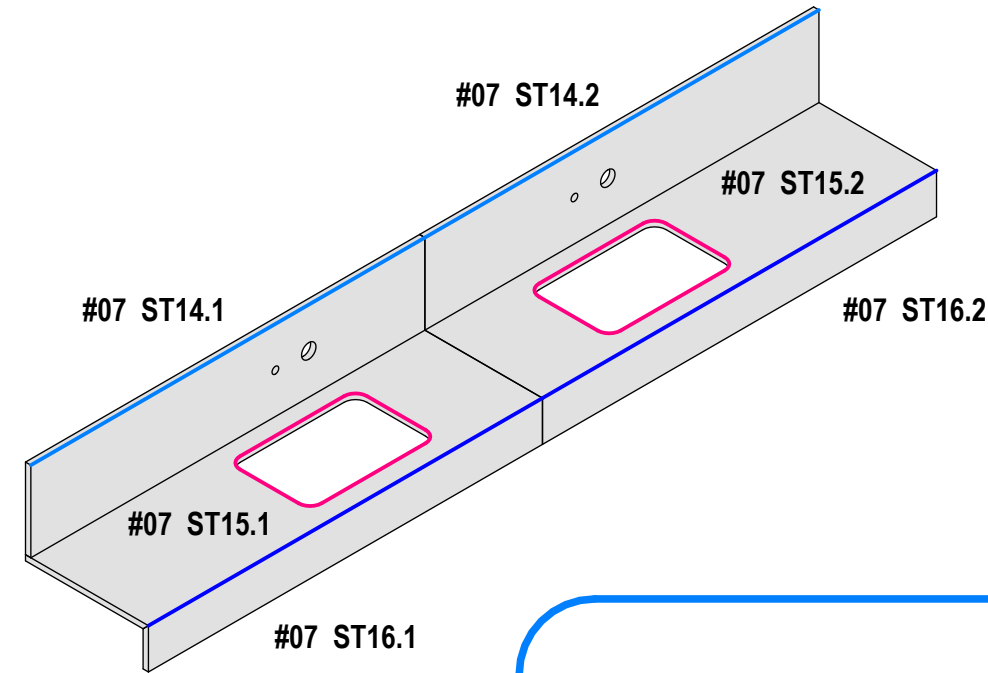
L1 BED 7 - MARBLE COUNTERTOP 3D VIEW
