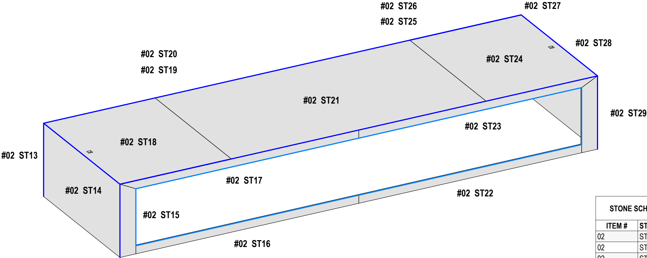
J02 - BUFFET COUNTER - 3D VIEW *REFER TO THE FOLLOWING PAGE FOR DETAILS. (Y26-N-2B - SW02B - BUFFET COUNTER)
